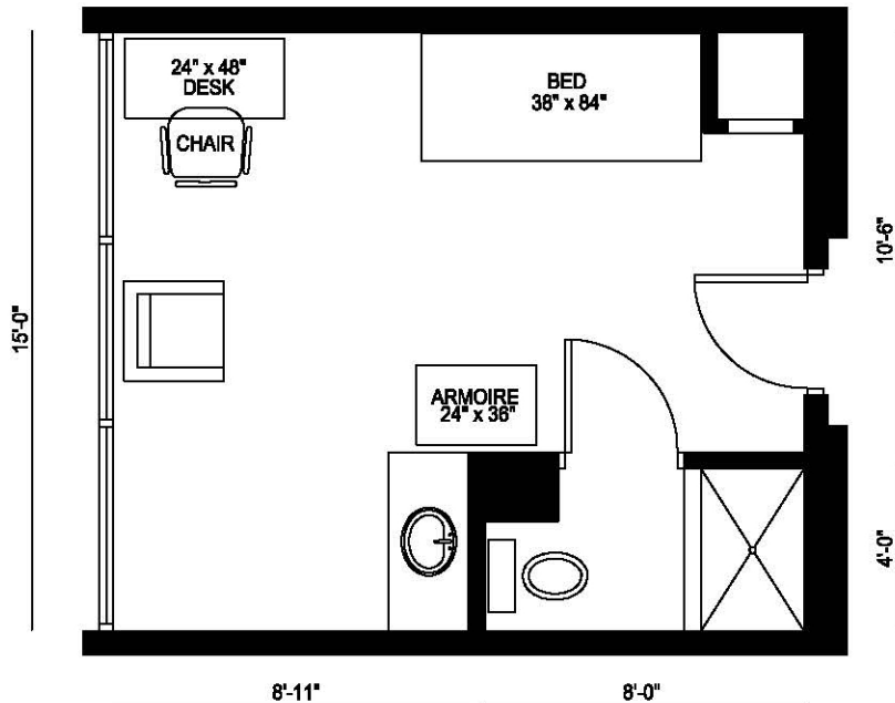
MORSANI HALL - FLOORPLAN G
