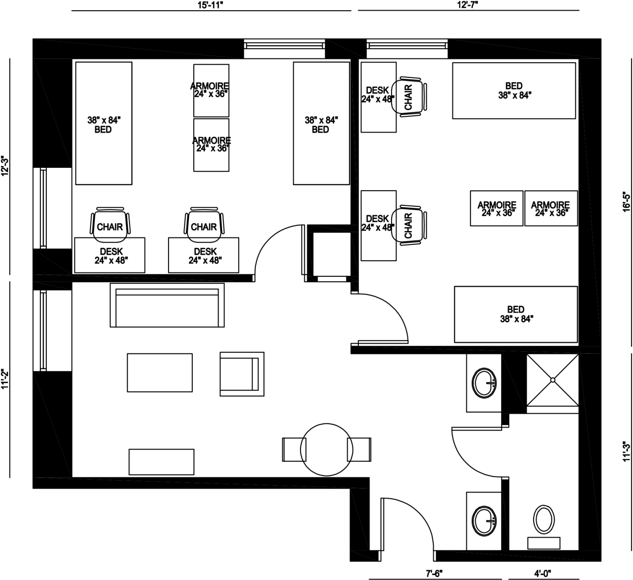
MORSANI HALL - FLOORPLAN B
