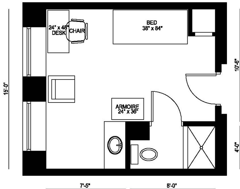
MORSANI HALL - FLOORPLAN A
